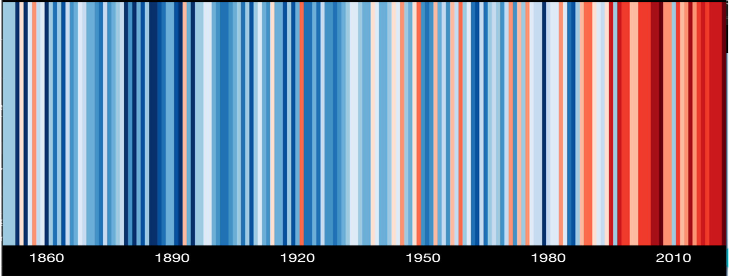
Temperature change in Ireland since 1850
